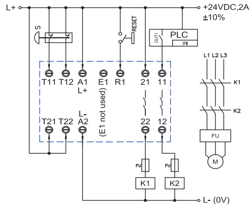
E-STOP dual-channel inputs without detection of shorts across contacts Category 3 / PL d
