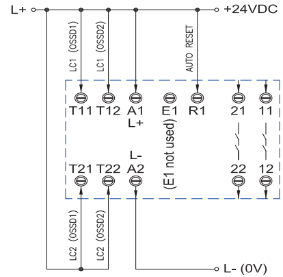
Dual-channel inputs for light curtain or photoelectric sensor, detection of shorts contacts via ESPE equipment Category 3 / PL d
