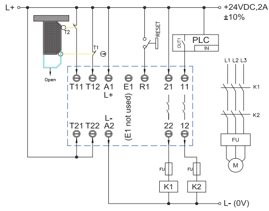
Safety door dual-channel inputs without detection of shorts across contacts Category 3 / PL d
