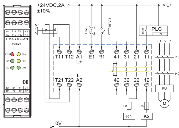
E-STOP dual-channel inputs with detection of shorts contacts Category 4 / PL e
