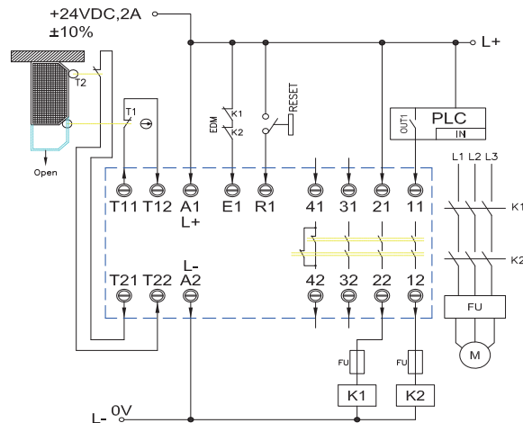
Safety door dual-channel inputs with detection of shorts contacts Category 4 / PL e
